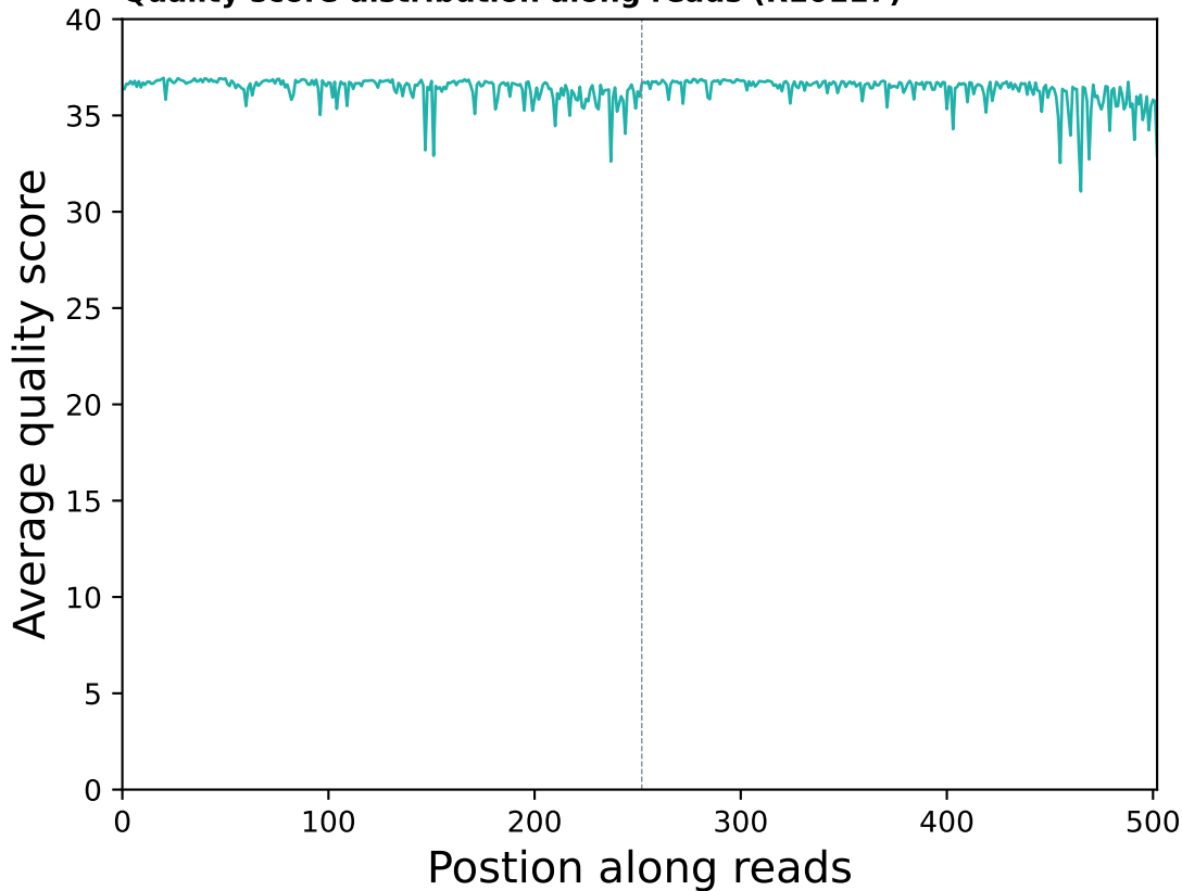
Quality score distribution along reads (R10117)
